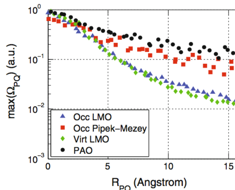
Graphene (delocalized)
