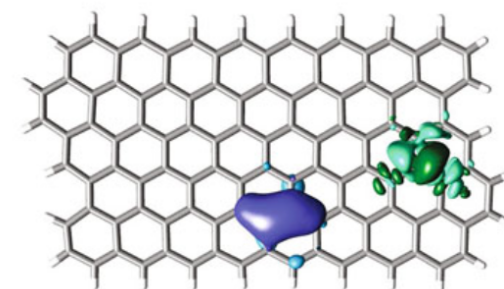
Graphene (delocalized)
